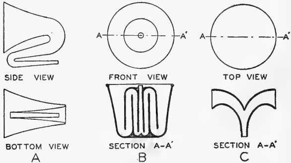
FIG. 8.21. Folded horns.
